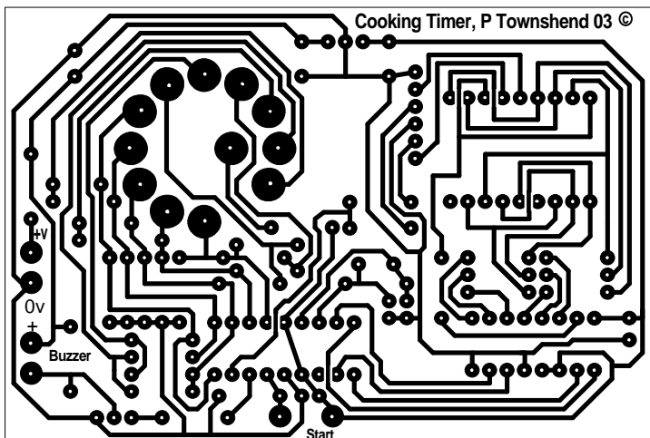
Underside track layout viewed from below
