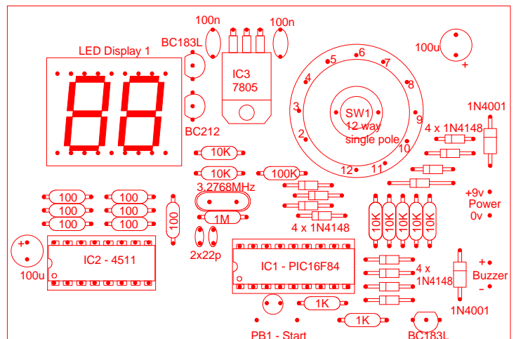
Component layout.
